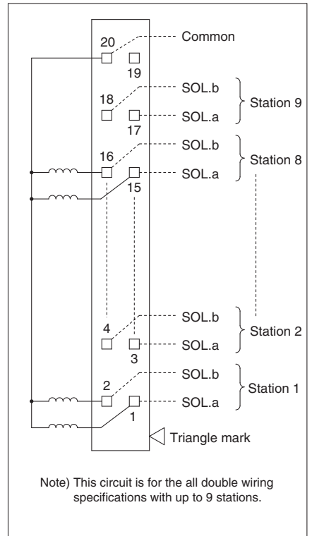
Type 60LPG: Flat ribbon cable (20 pins)
