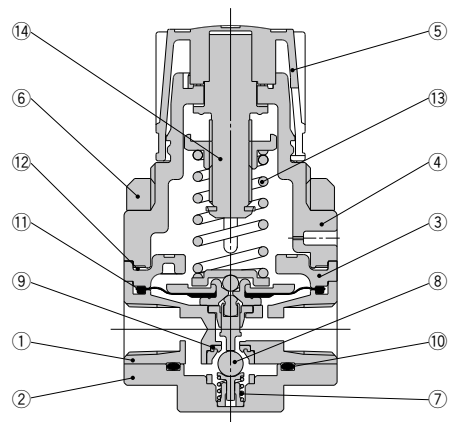
Component parts
