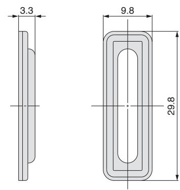
Size 26 mm
