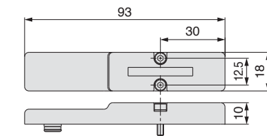
Size 18 mm
