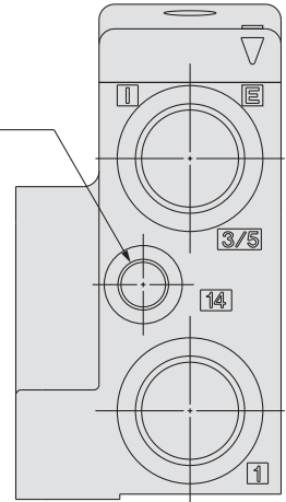
External pilot
