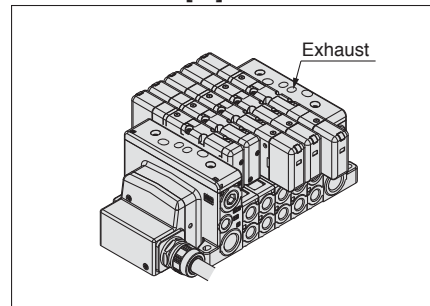
Direct EXH outlet with built-in silencer [-S]
